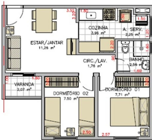
APART. 2 DORM. (45,39 m 2 ) ESCALA 1:50
